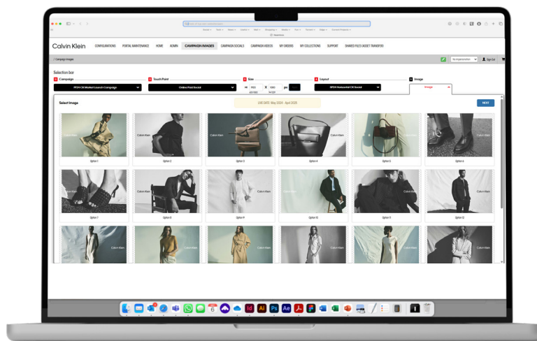
BannerBuilder
