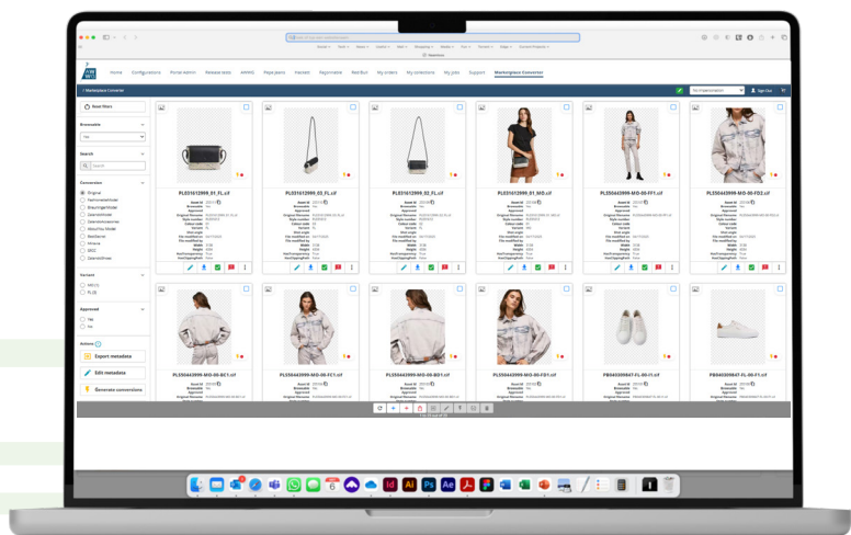
Marketplace Converter
